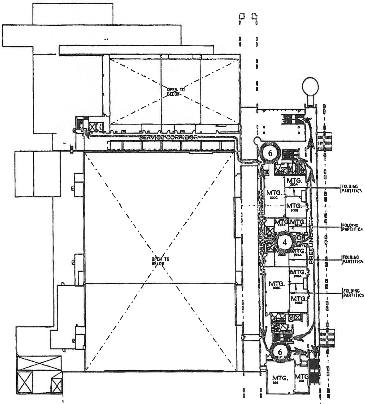
SECOND FLOOR - ALTERNATE EVACUATION ROUTES (NUMBERS REFER TO SECTION MONITOR ASSIGNMENT)
